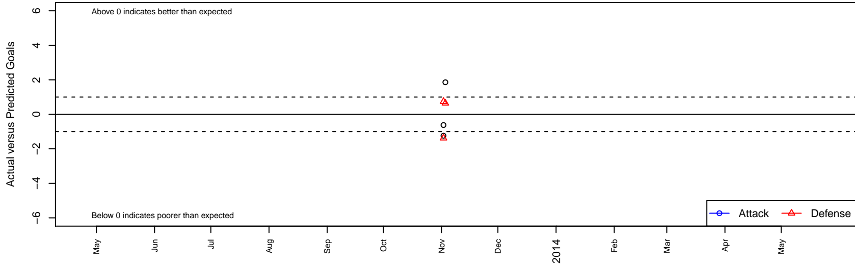
Infinity SC 00 Premier G99 Dots are actual minus expected GF (blue circles) and GA (red triangles). Blue line is smoothed change in attack strength. Red is smoothed change in defense strength.
